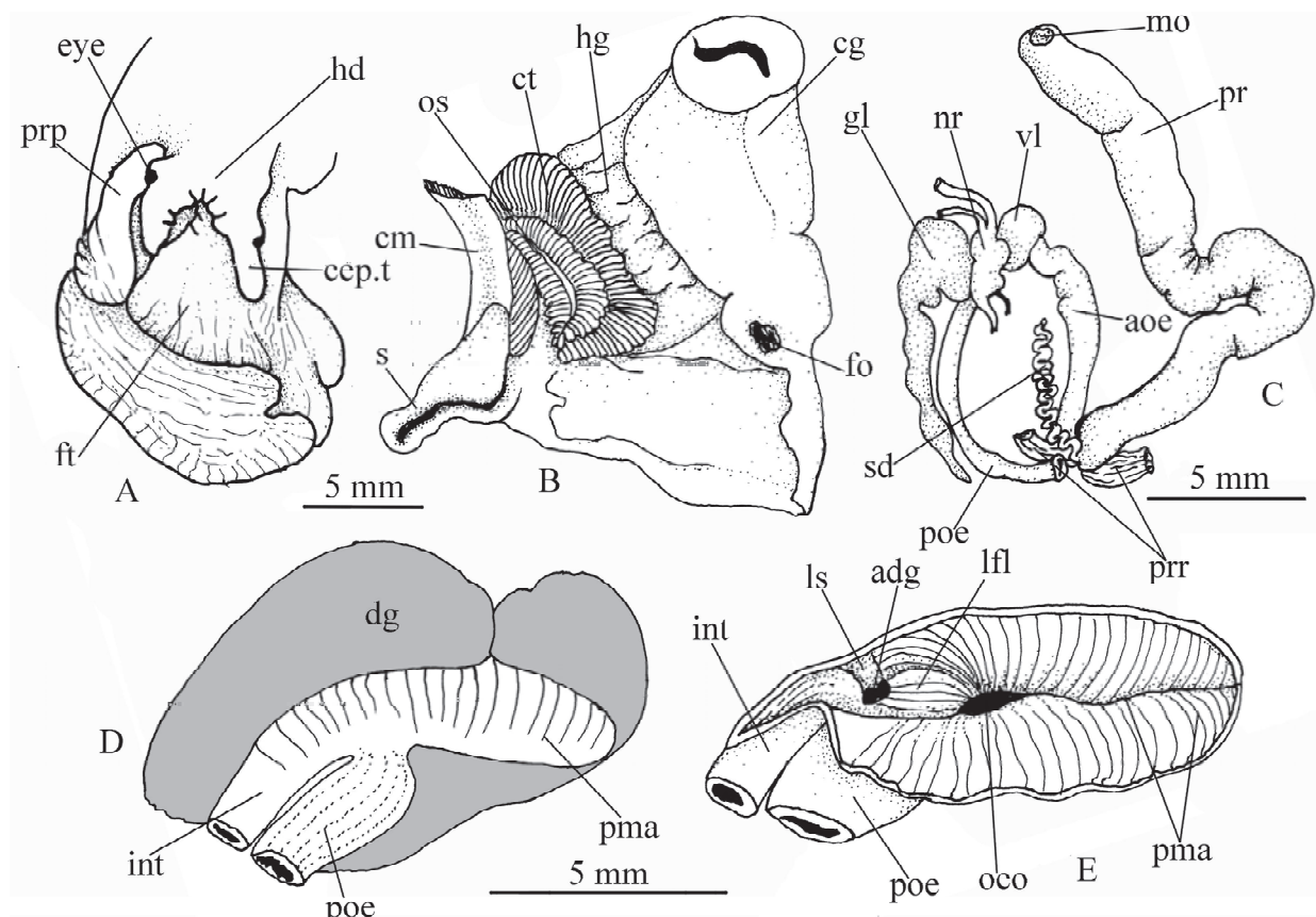
FIG. 18. Anatomy of Aulacofusus gulfini sp. n., paratype (shell – Fig. 17B, radula – Fig. 16D): A – cephalopodium, front view; B – mantle; C – foregut (salivary glands not shown); D – stomach, general view; E – opened stomach.
